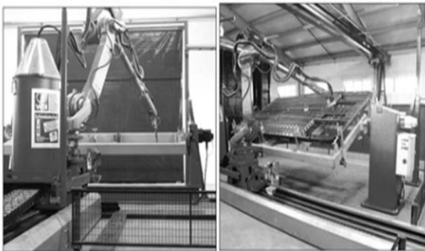
Fig. 6. Industrial robots – welding application
