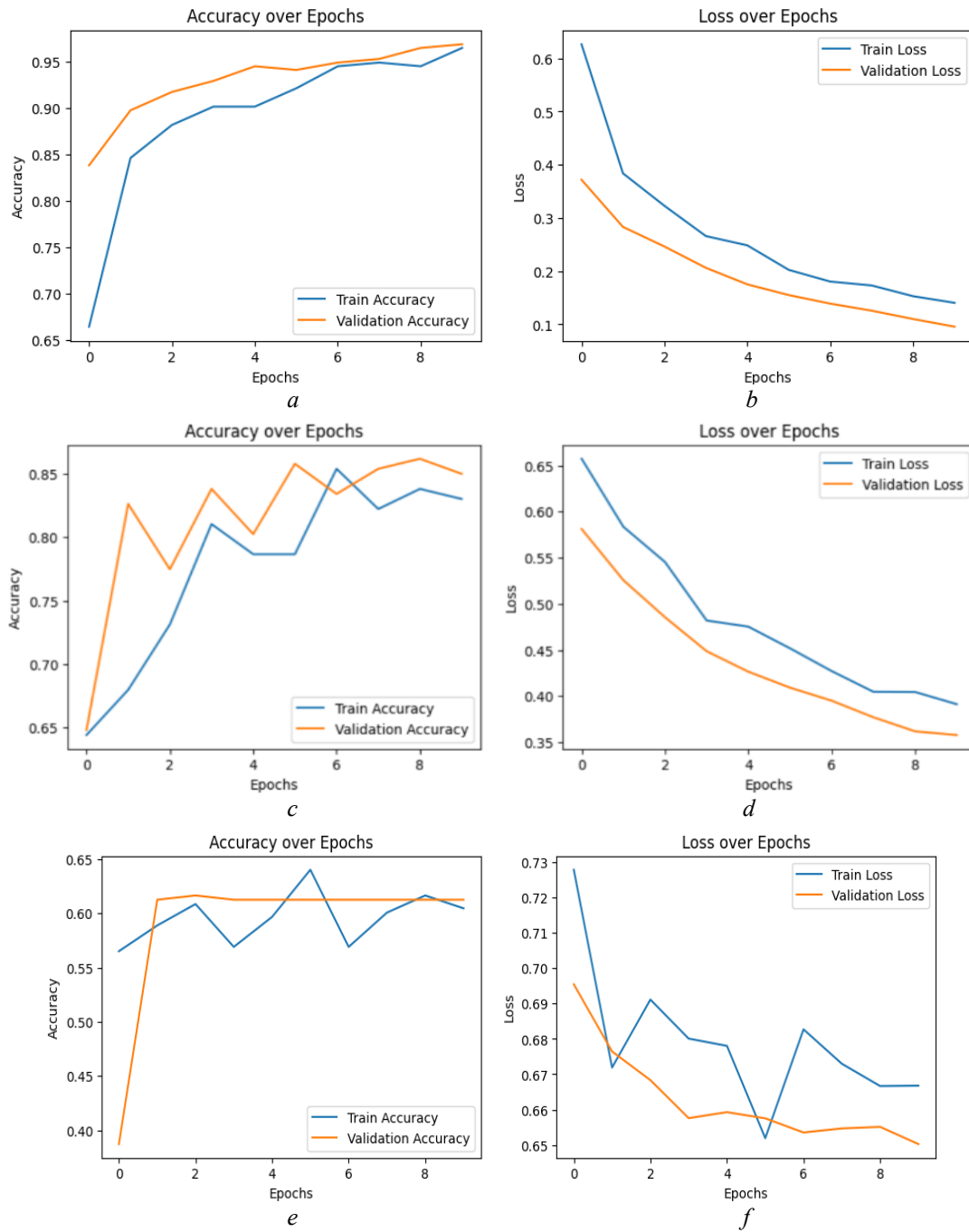
Fig. 4. Accuracy and Loss for transfer-learning models:
