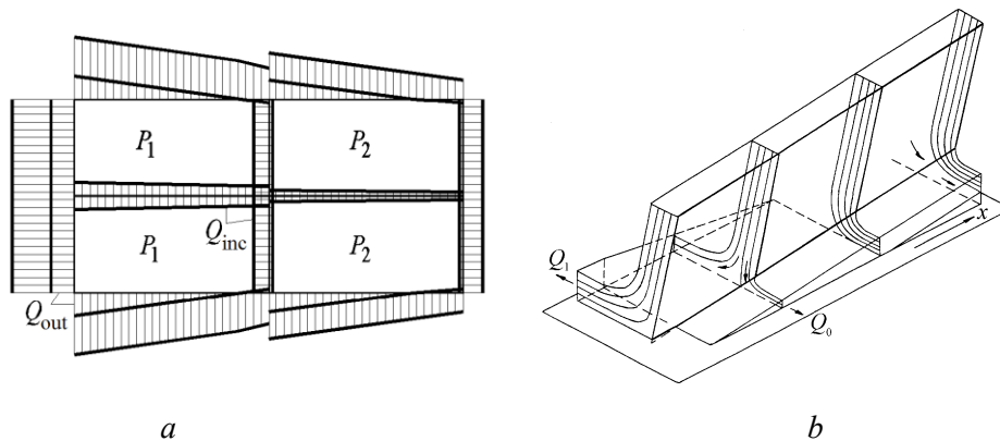
Fig. 1 Hovercraft schematic:
